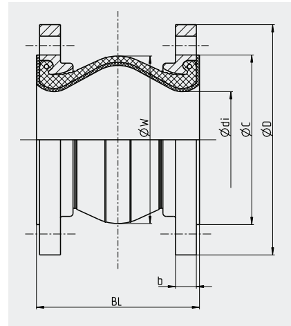
Type Ai-1 Universal expansion joint with PTFE lining and PTFE supporting ring
